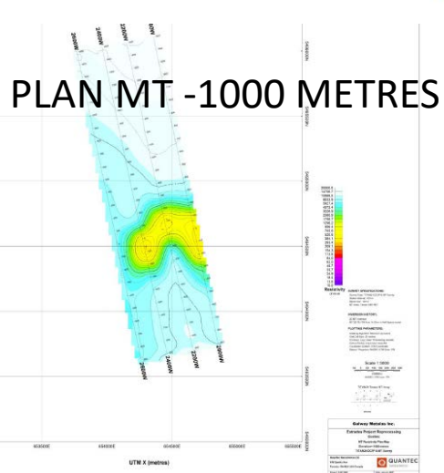
Figure 4-18: MT resistivity model, -1000 m elevation.
